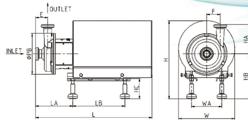
衛生級離心泵尺寸圖 SCP Series pump dimension
