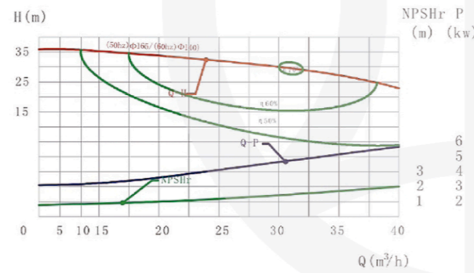
SCP-20-1 (Q-H曲線圖/Graph)
