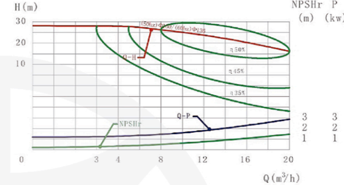
SCP-15 (Q-H曲線圖/Graph)
