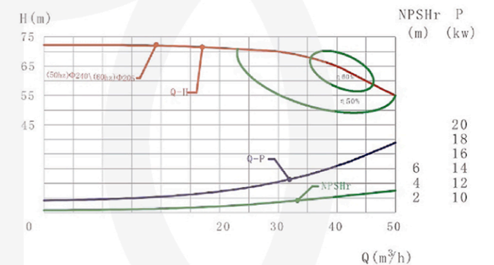
SCP-35-2 (Q-H曲線圖/Graph)
