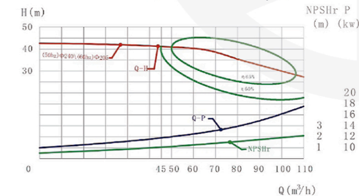
SCP-40-1 (Q-H曲線圖/Graph)
