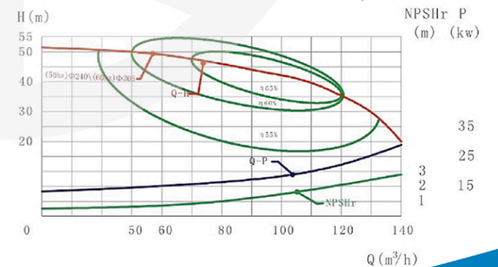
SCP-40-2 (Q-H曲線圖/Graph)
